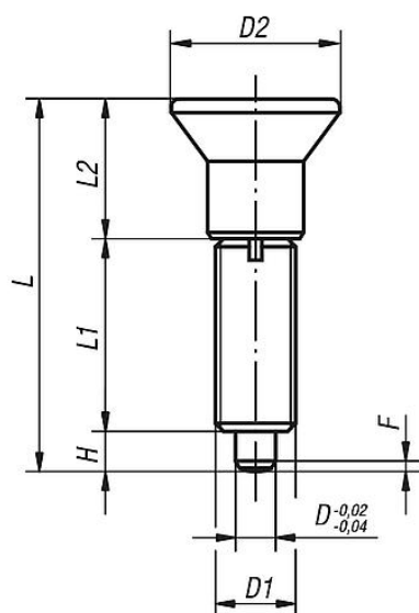
Form G without locknut
