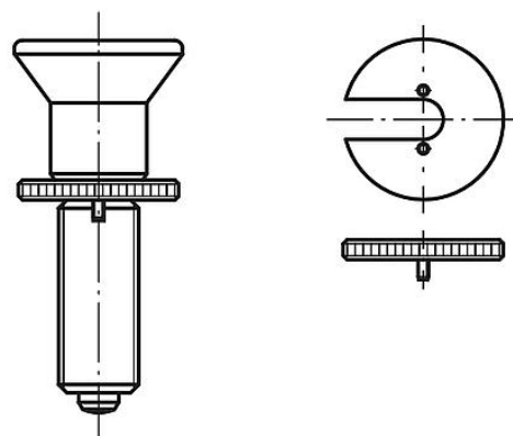
Indexing plunger with screw-in washer
